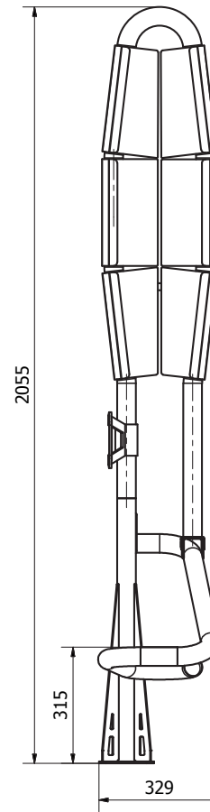
ACCP_VH-V1.006 Front Elevation
