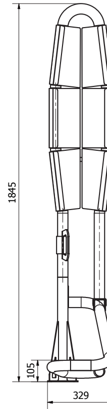
ACCP_VL-V1.006 Front Elevation
